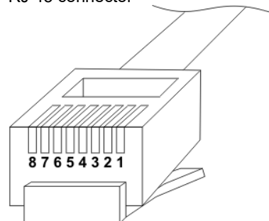
RJ 45 connector
