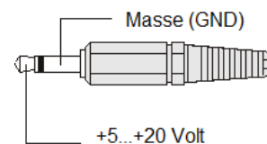
Connector assignment (3.5 mm barrel plug)
